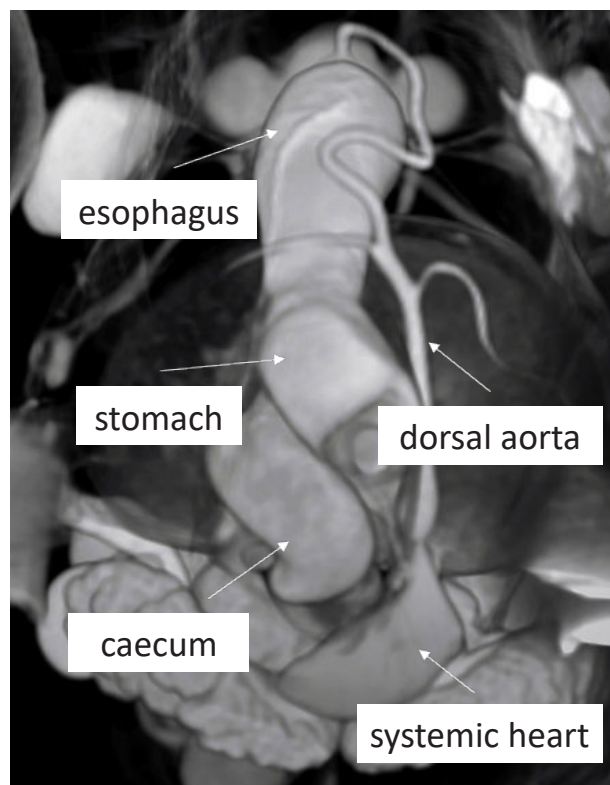
Figure 5. Volume rendering of Emperor dumbbo octopus viscera, ventral view, with anterior facing up. (Credit: Ziegler and Sagorny, BMC Biology, 2021) [2]
